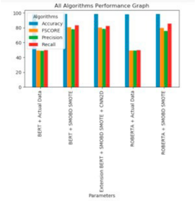
Fig. 2: Performance evaluation of various algorithms across different datasets
